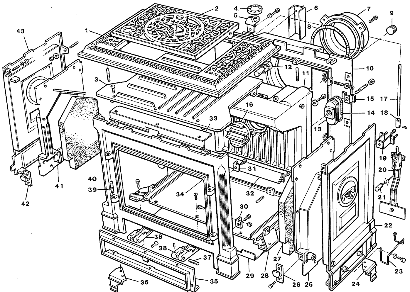
COALBROOKDALE DARBY STOVE - BOILER MODEL MAIN BODY ASSEMBLY
