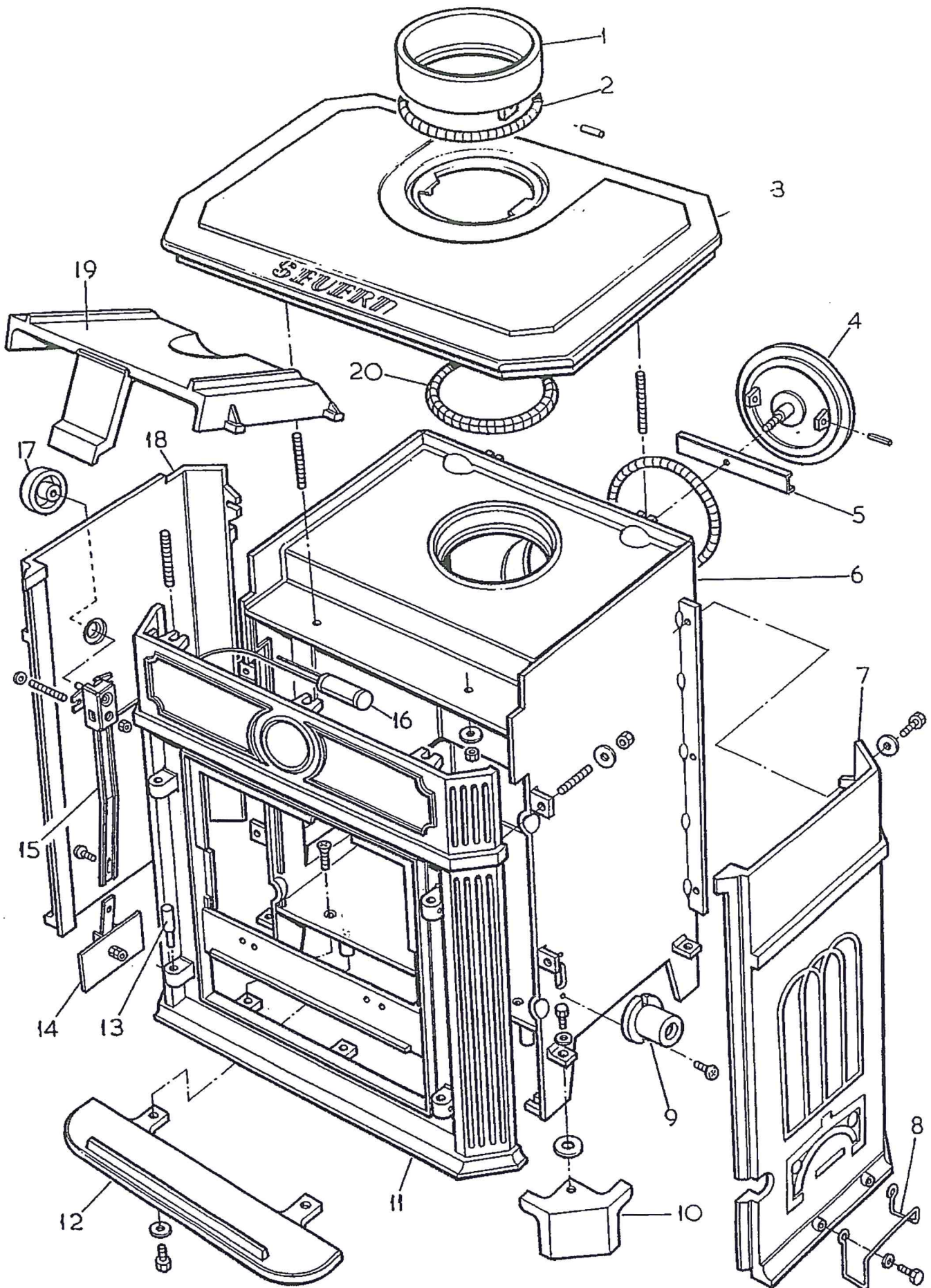
COALBROOKDALE SEVERN STOVE (BOILER) MAIN BODY ASSEMBLY
