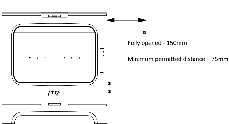
Minimum right side clearance distance, to accommodate the extended Bypass Boss
